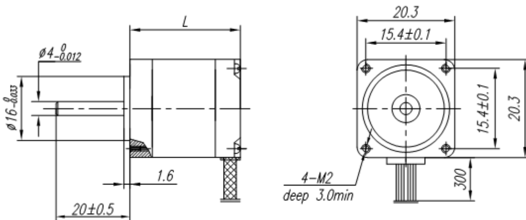
Mechanical Dimensions(外形图): unit=mm
