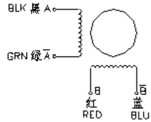
BI-POLAR(4LEADS)
