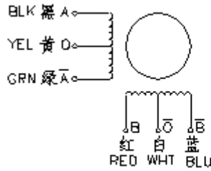
UNI-POLAR(6 LEADS)
