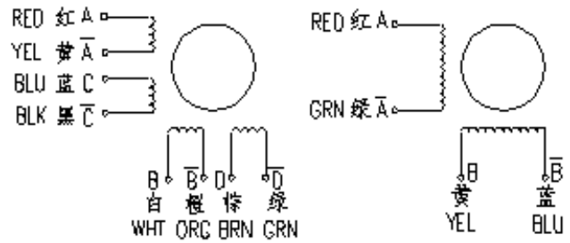
UNI/BI-POLAR(8 LEADS)
