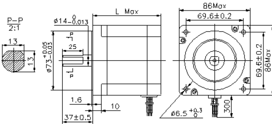
Mechanical Dimensions(外形图): unit=mm
